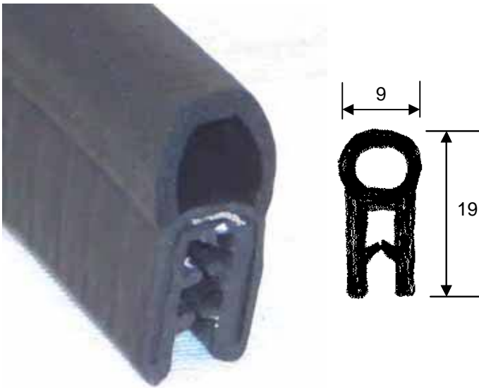
EDGE SEAL #TRME Black rubber. For boot edge lips etc. Overall 19mm high. 9mm diameter soft round hollow bead. For up to 3mm thick panels. Steel reinforced 'U'. £3.50/mtr (£4.11 inc vat)
