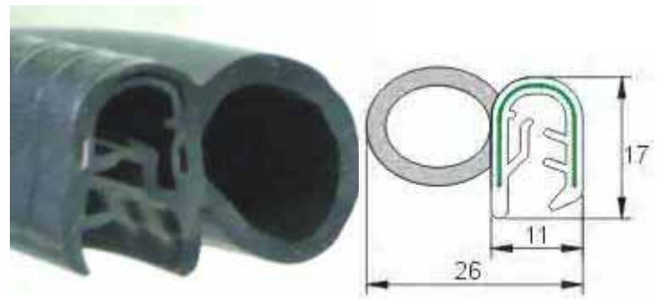
DOOR SEAL #TRMDR Suitable for GRP panels up to 5mm thick. Sponge tube 17mm diameter bonded to steel-reinforced PVC gripper with leather-grain finish. £3.50/mtr (£4.11 inc vat)
