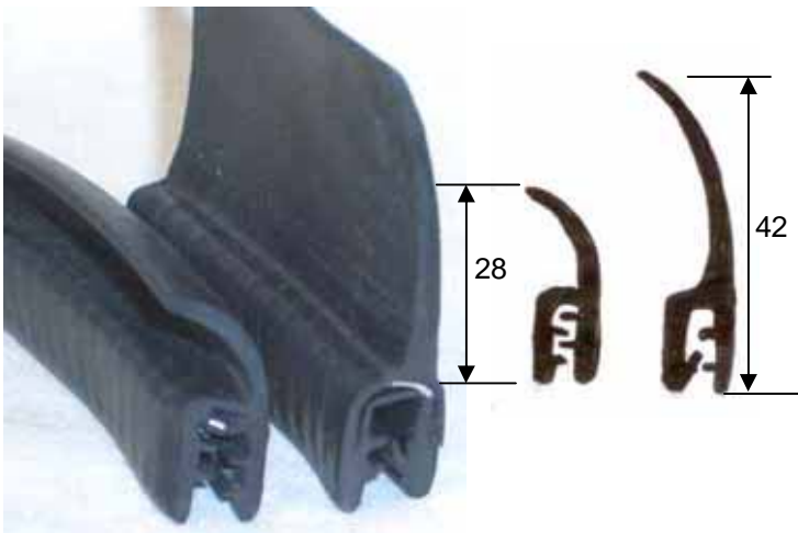
BOOT & DOOR SEAL Steel reinforced 'U' section SMALL #TRMBS 28mm total height for up to 3mm panels. LARGE #TRMBL 42mm total height for up to 5mm panels. Both £4/mtr (£4.70 inc vat)
