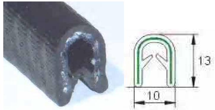
EDGE TRIM #TRMPV Patterned PVC with steel reinforcing. Max panel thickness 5mm. Channel depth 10mm. Will form to 50mm radius. £2.50/mtr (£2.93 inc vat)
