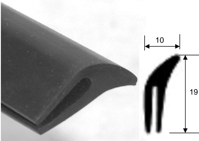
LEAF SEAL #TRML1 Black flexible rubber. For window seal, boot edge lips etc. Overall 19mm high. For up to 2mm thick panels. £3.50/mtr (£4.11 inc vat)
